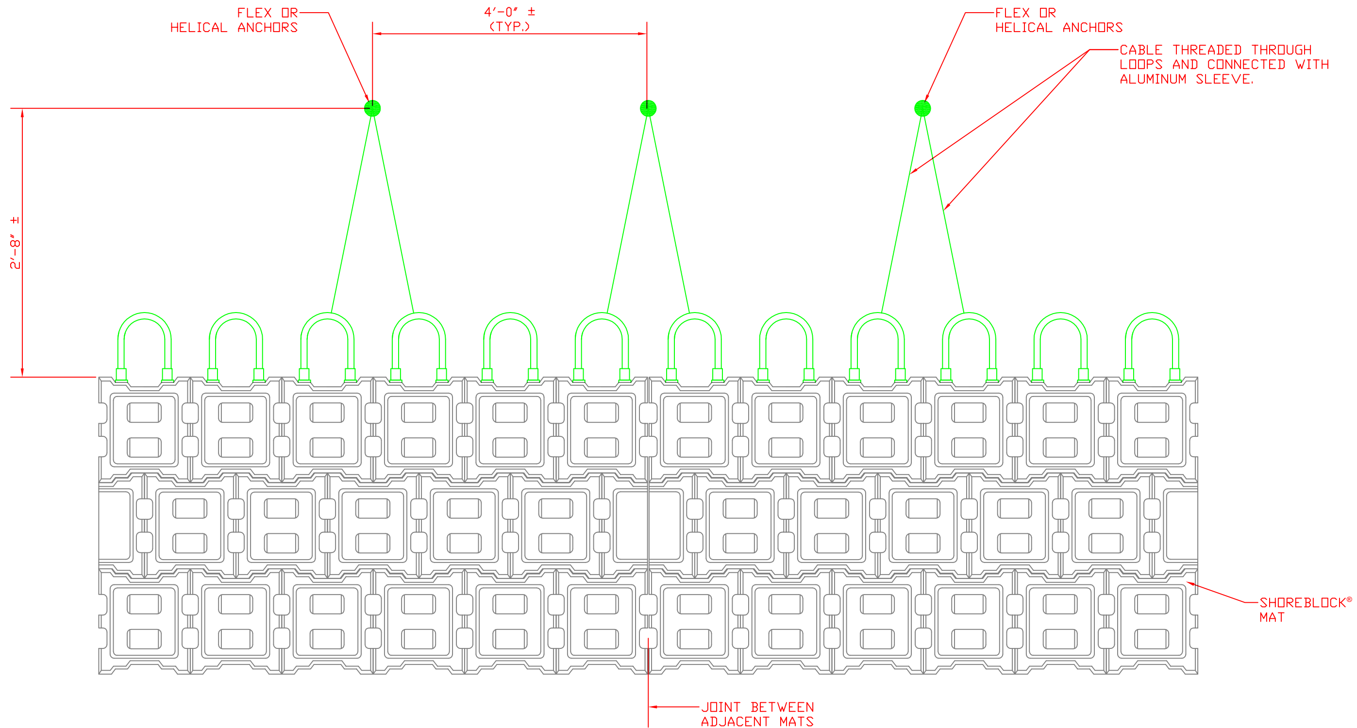
PLAN VIEW
