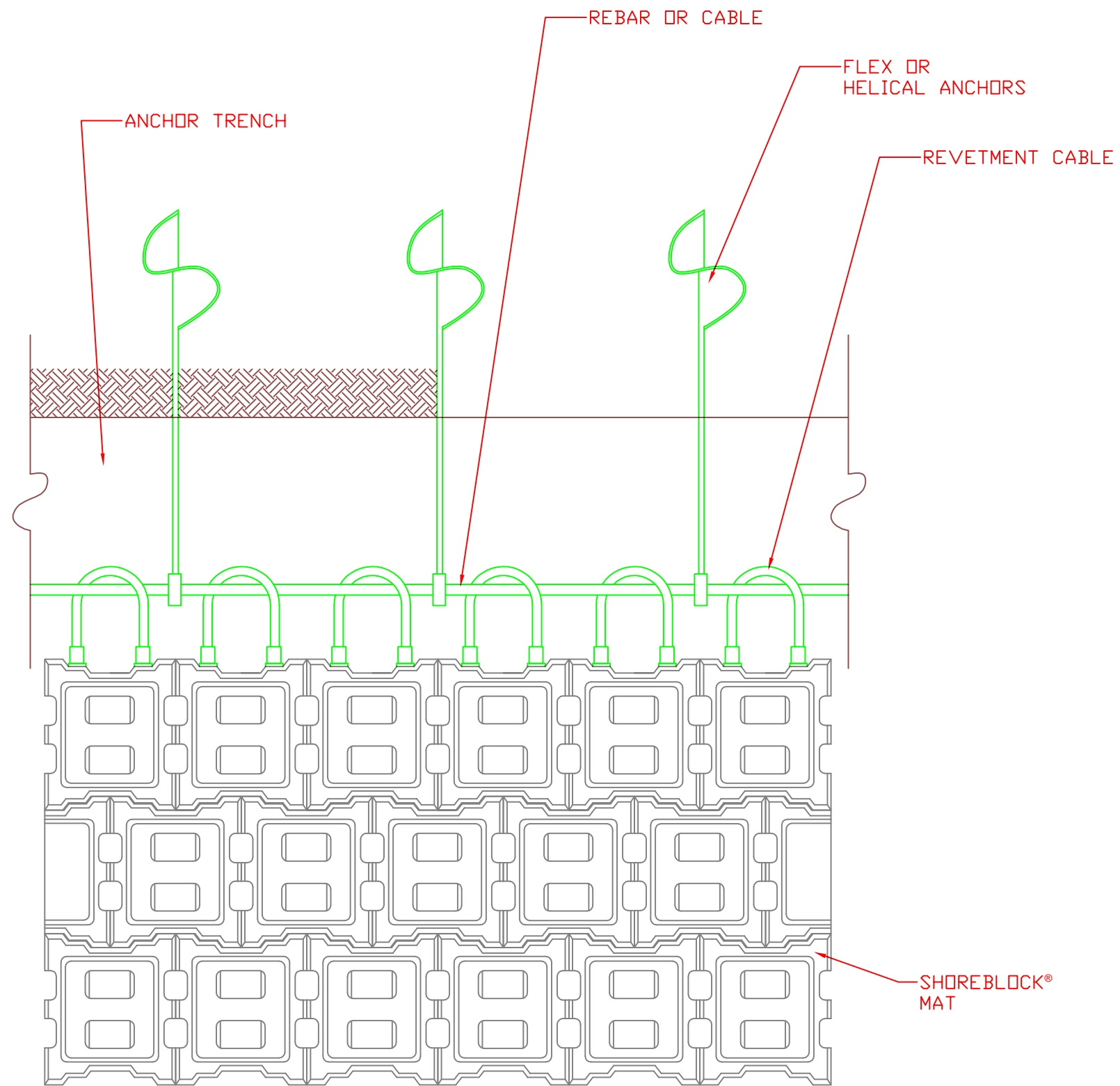
PLAN VIEW
