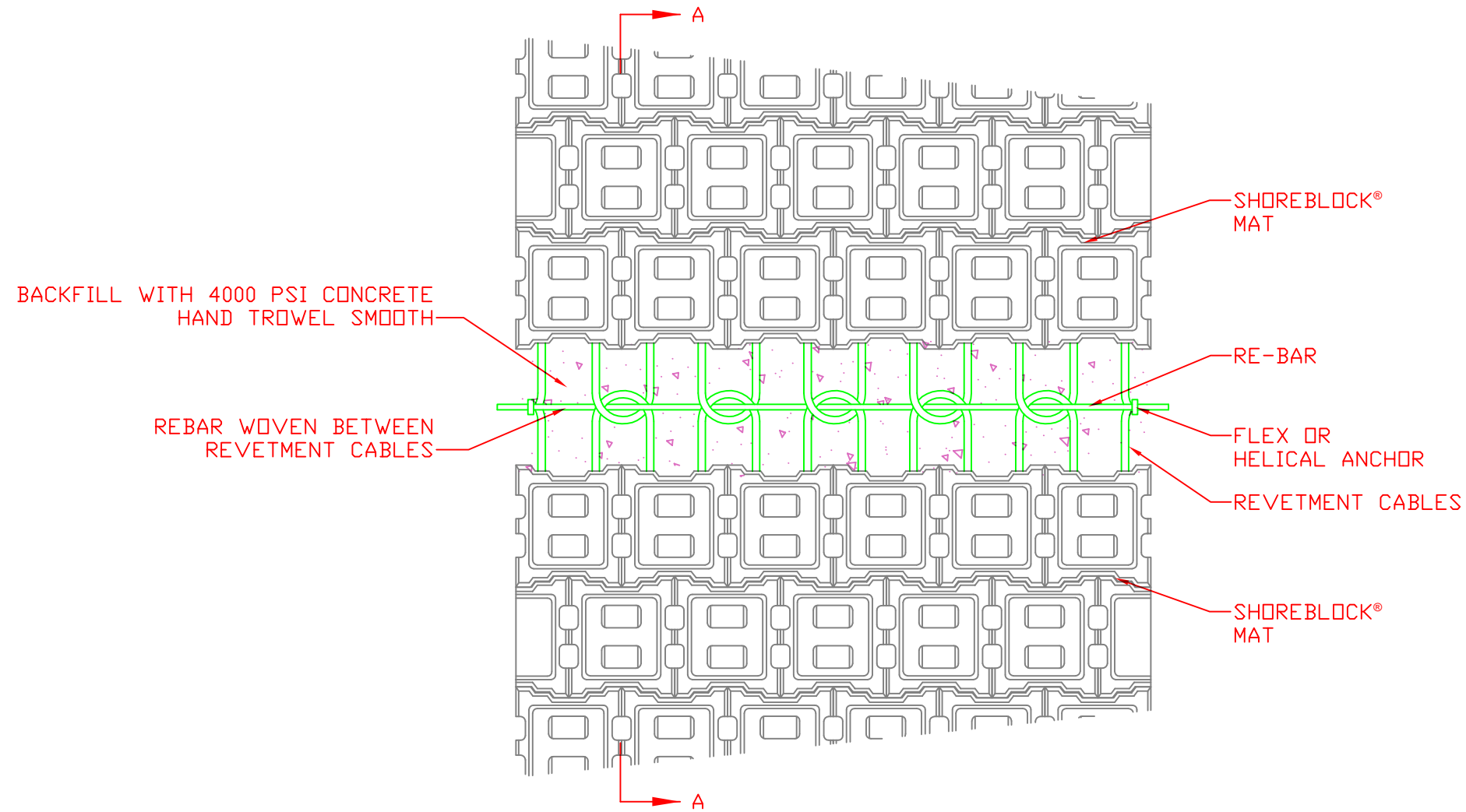
PLAN VIEW
