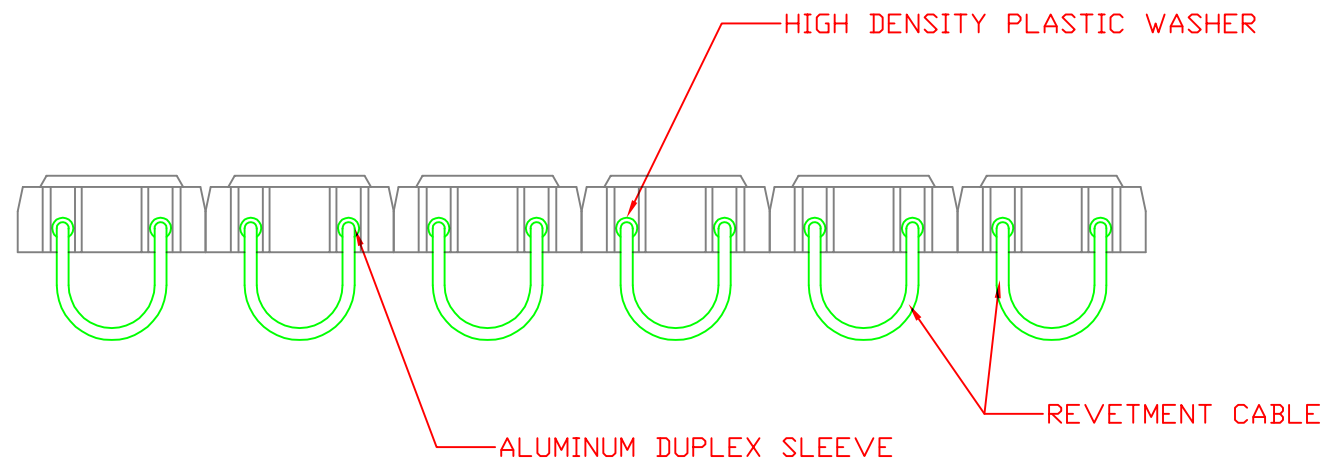
END VIEW
