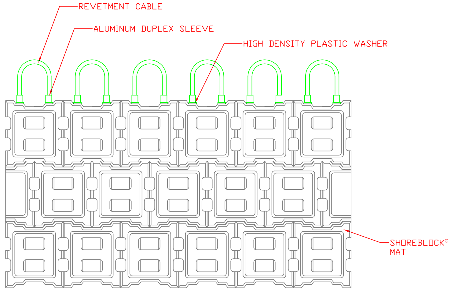
PLAN VIEW
