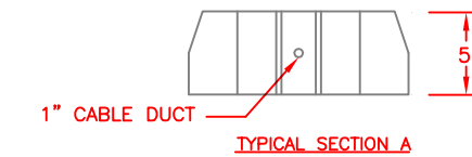
TYPICAL SECTION A
