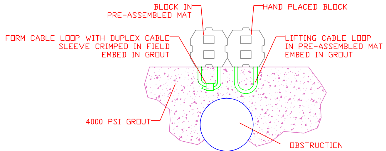
LONGITUDINAL (LIFTING) CABLE CONNECTION TO GROUT DETAIL A
