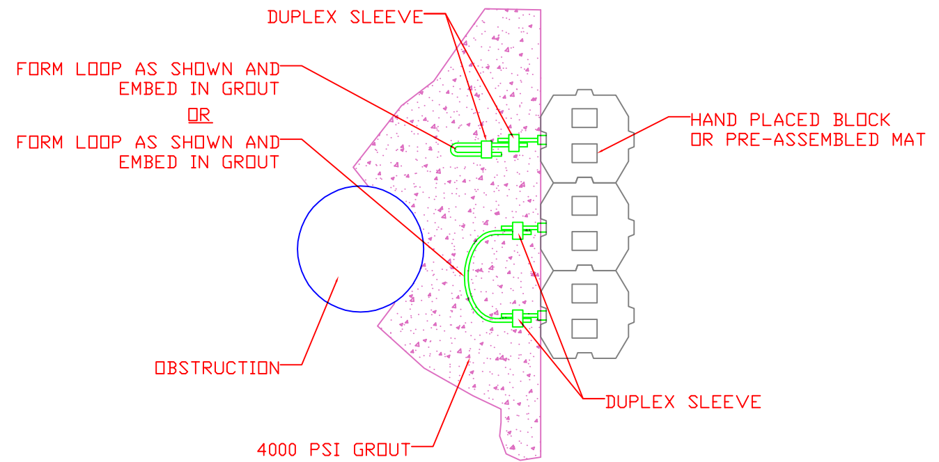
LATERAL CABLE CONNECTION TO GROUT DETAIL B
